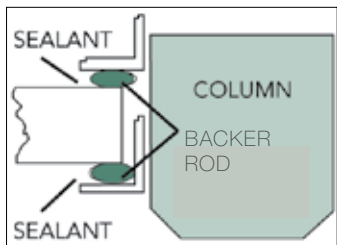
CURTAIN WALL CONSTRUCTION
